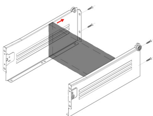
Back panel assembling
