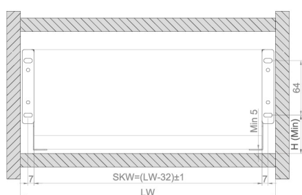
Cabinet space requirements and mounting dimensions
