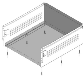
Bottom panel assembling
