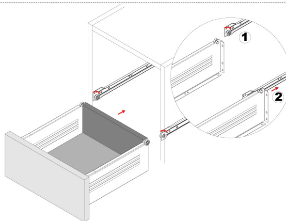
Installing the drawer into the cabinet
