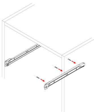
Fixing slides to the cabinet
