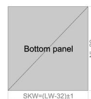
Cutting dimensions of MDF
