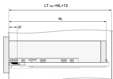
Standard drawer
