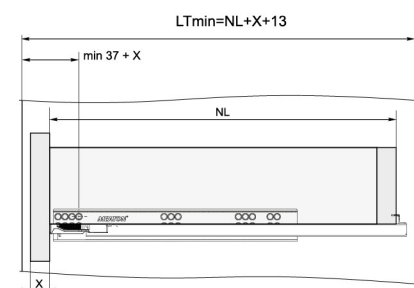
Built-in drawer
