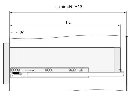
Standard drawer
