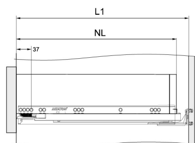
Standard drawer
