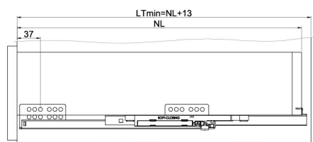
Standard drawer
