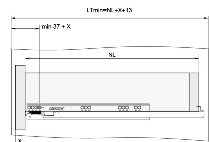
Built-in drawer
