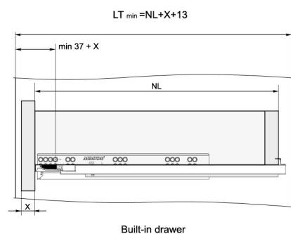
Built-in drawer
