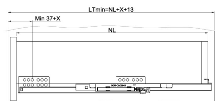
Built-in drawer
