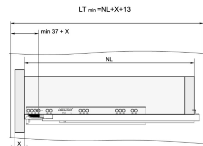
Built-in drawer
