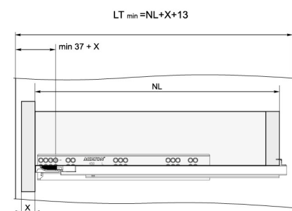
Built-in drawer
