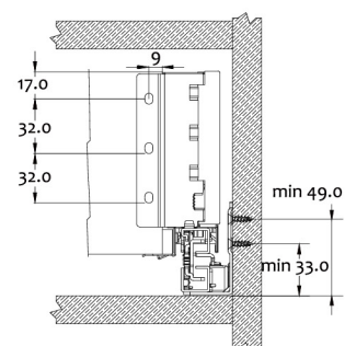
Back panel installation dimensions
