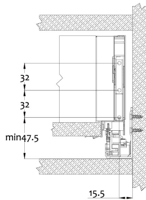
Back panel installation dimensions
