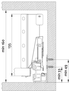
Drawer slide installation dimensions
