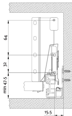
Drawer slide installation dimensions
