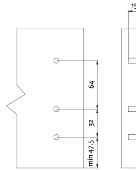
Cutting dimensions for back panel
