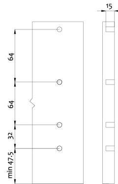
Cutting dimensions for back panel
