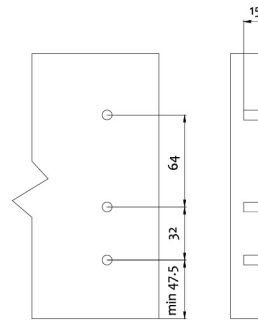
Cutting dimensions for back panel
