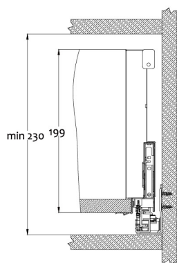
Drawer slide installation dimensions
