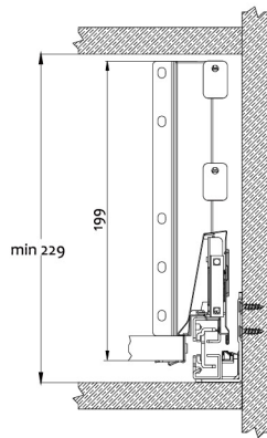
Cabinet space requirements
