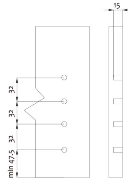
Cutting dimensions for back panel
