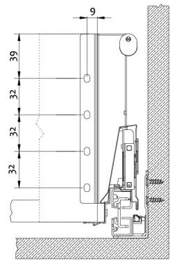
Back panel installation dimensions
