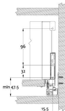
Drawer slide installation dimensions
