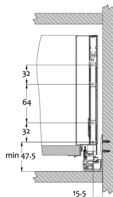
Drawer slide installation dimensions
