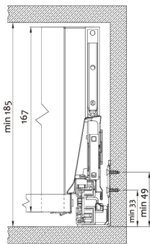
Drawer slide installation dimensions
