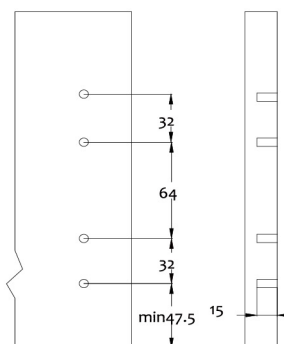
Cutting dimensions for back panel
