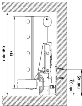
Drawer slide installation dimensions
