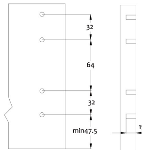
Cutting dimensions for back panel
