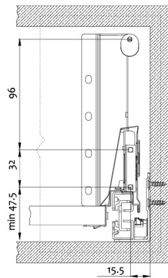
Front connector panel installation dimensions
