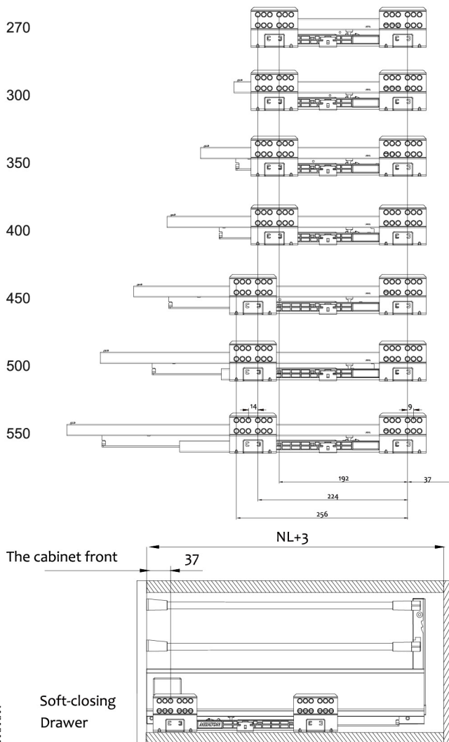
Drawer slide installation dimensions
