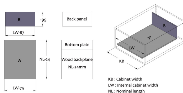
Cutting dimensions for back panel
