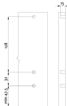
Cutting dimensions for back panel
