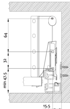
Drawer slide installation dimensions
