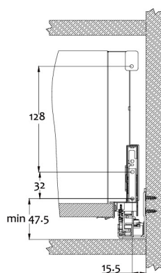
Drawer slide installation dimensions
