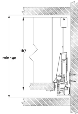
Cabinet space requirements
