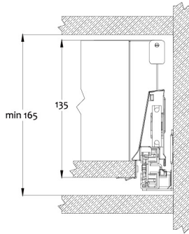
Cabinet space requirements
