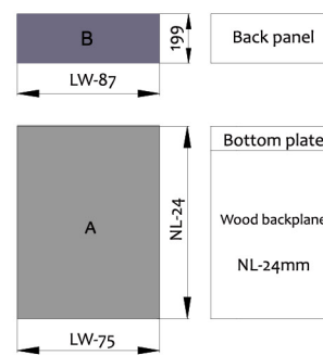
Cutting dimensions for back panel
