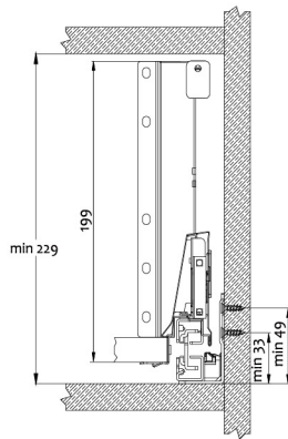
Cabinet space requirements
