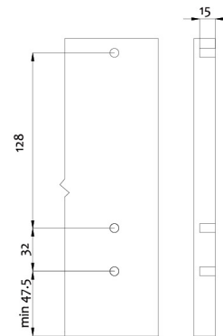
Cutting dimensions for back panel
